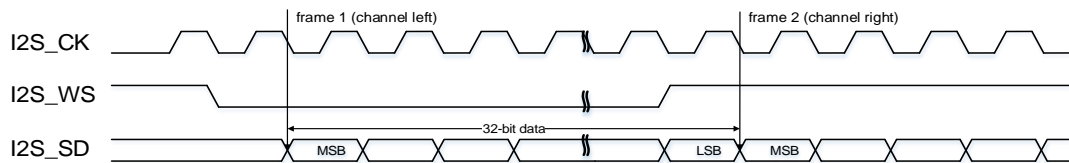
Figure 18-14. I2S Phillips standard timing diagram (DTLEN=10, CHLEN=1, CKPL=0)
