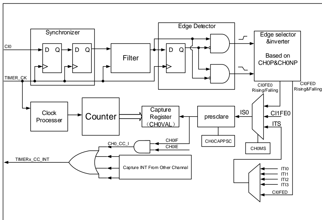
Figure 15-42. Input capture logic
