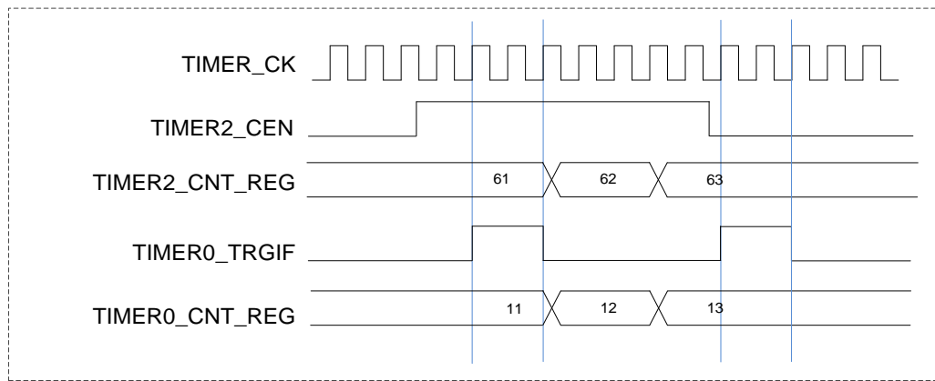
Figure 15-31. Pause TIMER0 with enable signal of TIMER2
